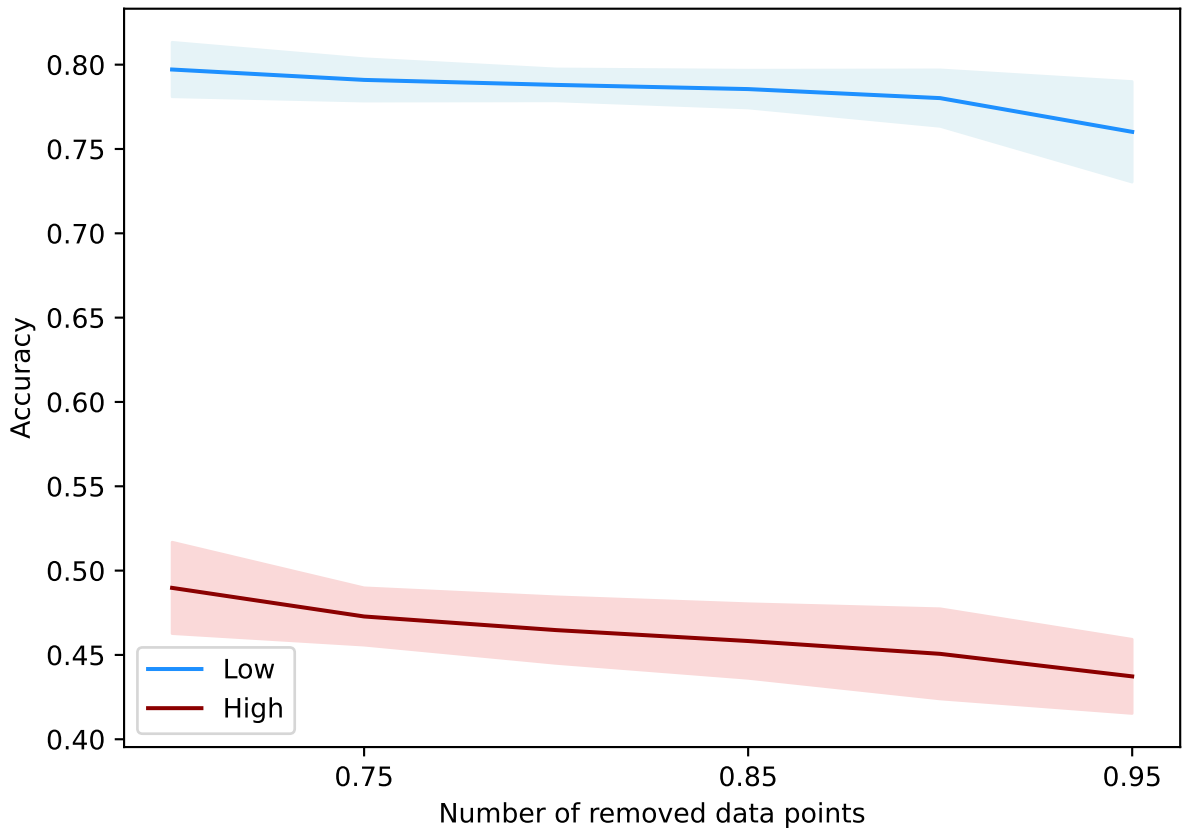
DataAttrOpt(10000, 0.2, 15, best, +b, alpha=best) - imdb-embeddings
